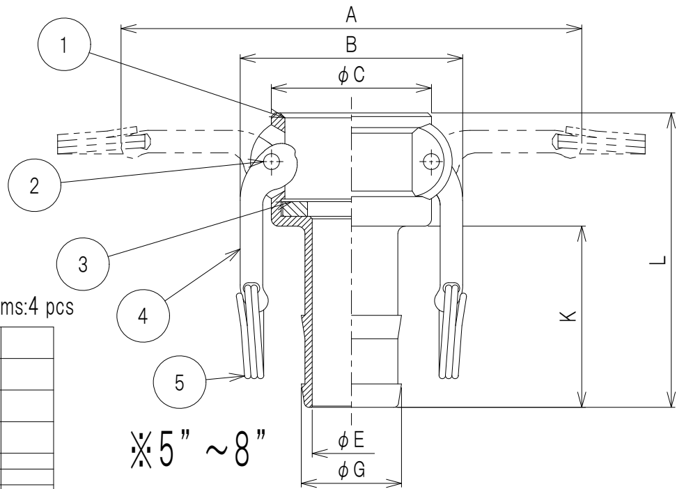
6 3 3 - C A L DIMENSION TABLE BY SIZES (UNIT:mm)
