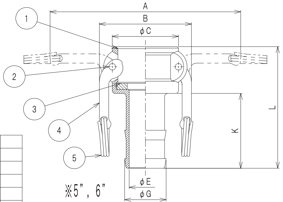
6 3 3 - C S S T DIMENSION TABLE BY SIZES (UNIT:mm)
