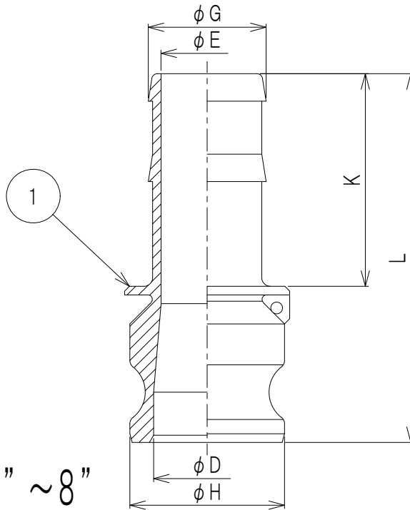
6 3 3 - E A L DIMENSION TABLE BY SIZES (UNIT:mm)
